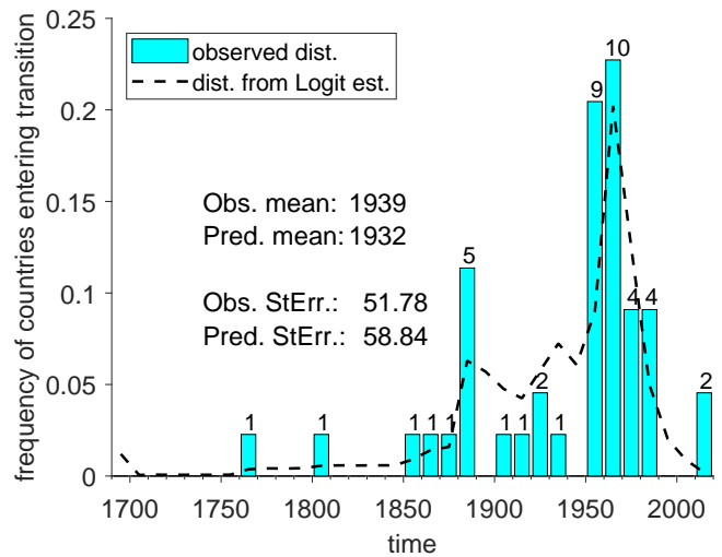
Figure 12: Distribution of transition dates, Spec. (9)
