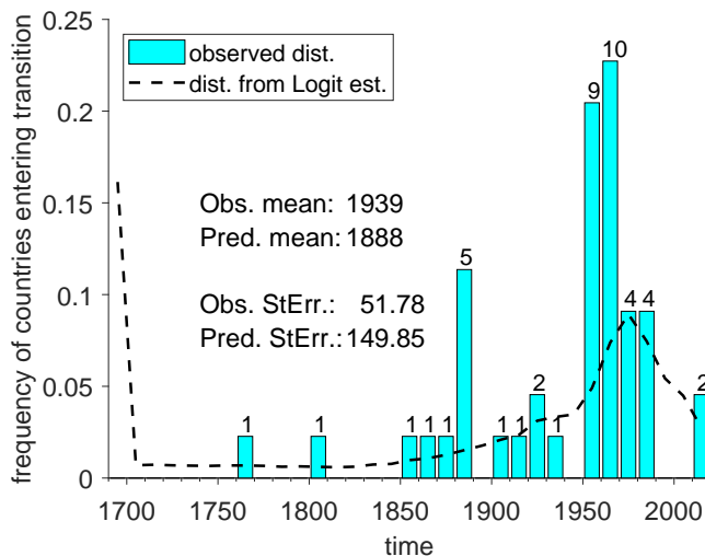
Figure 10: Distribution of transition dates
